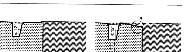
⑩ 'Zurich' gutter
